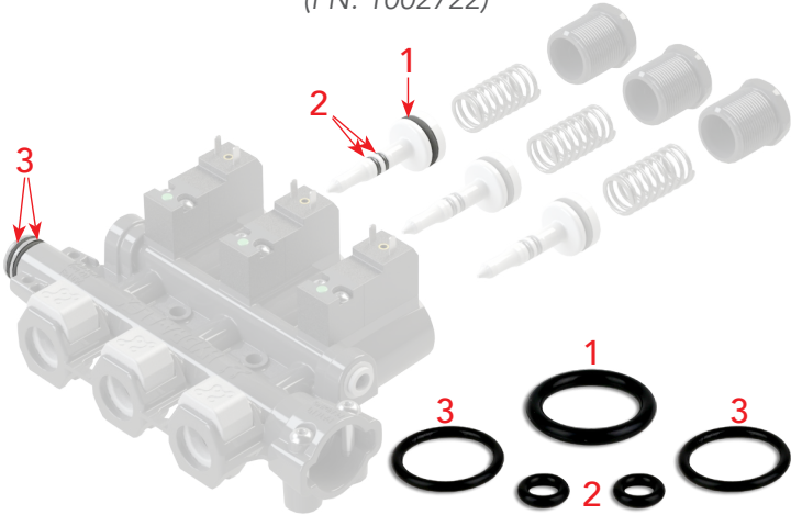
SAM O-RING REPAIR KIT (PN: 1002722)
