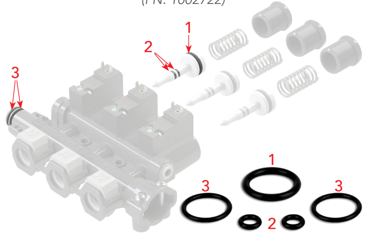
SAM O-RING REPAIR KIT (PN: 1002722)
